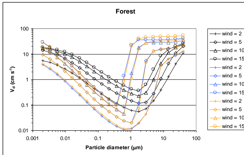
Figure 4-6. Comparison of particle dry deposition velocities as a function of size and wind speeds (m/s) for three models: black – Zhang et al. (2001); blue – Slinn and Slinn (1980); orange – AERMOD (EPA, 1998). Results are shown for a forest landuse category during daytime neutral stability. Particle density was set at 1.5 \text{ g/cm}^3 .
