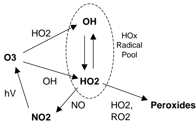
Figure 7-3. Daytime reactions of ozone with HOx (OH and HO 2 ) showing potential for reformation of ozone or ozone destruction via peroxide formation.
