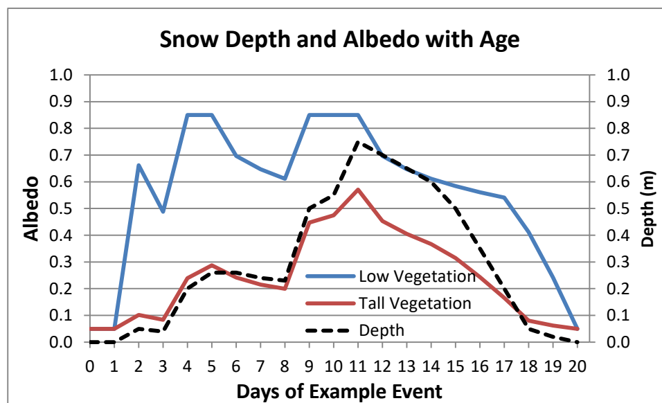
Figure 4-7. Example of grid-cell albedo evolution for a hypothetical 20-day springtime snow event (assuming ablation conditions) for low and tall vegetation grid cells with a terrestrial (non-snow) albedo of 0.05.
