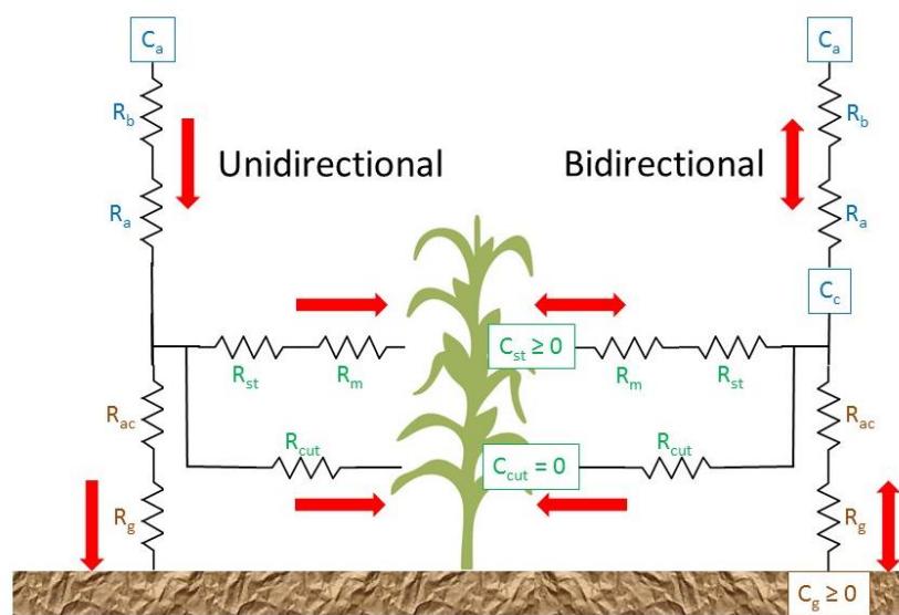
Figure 4-5. Right side shows a schematic of the bidirectional \text{NH}_3 deposition/re-emission scheme of Zhang et al. (2010) and Whaley et al. (2018); left side shows the original unidirectional deposition scheme of Zhang et al. (2003). Pathway resistances ( R ) and bidirectional compensation points ( C ) are shown.
