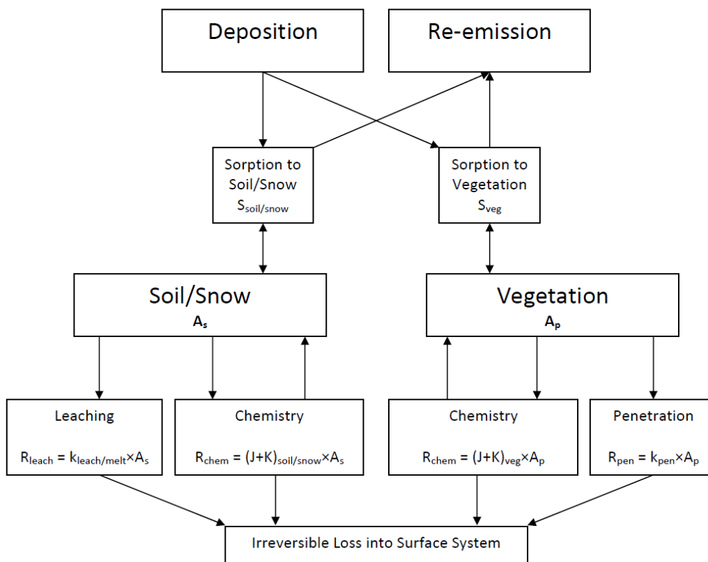
Figure 4-8. Schematic of the CAMx surface model.
